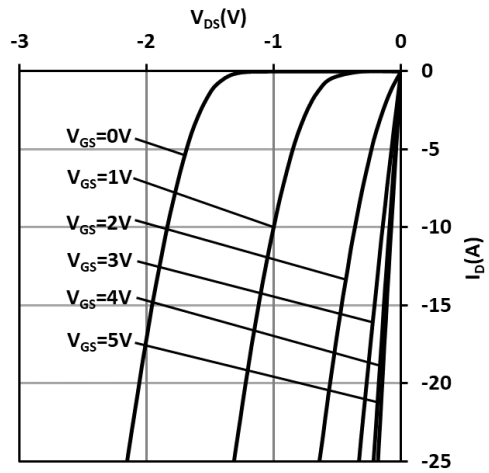
Fig. 8 Typ. Reverse Drain-Source Characteristics (VGS ≥ 0, Tj = 25°C)
