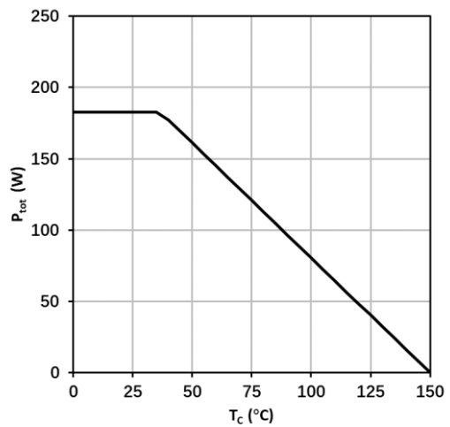
Fig. 16 Power Dissipation
